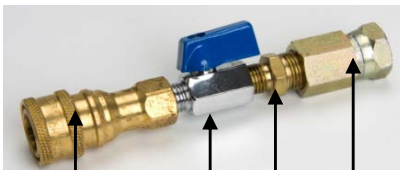
(Female) (Ball Valve) (Swivel) (Adapter) Pressure Inlet Assembly Part # PIAV12
